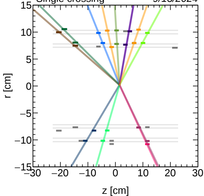
INTT Streaming readout Single crossing 9/13/2024
