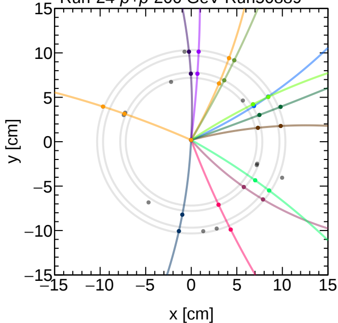
sPHENIX Preliminary Run-24 p+p 200 GeV Run50889
