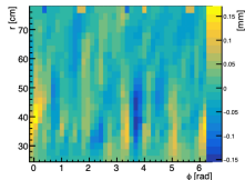
\rho component of int. distortion in xy plane at z=54.065
