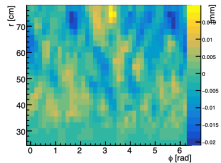
z component of int. distortion in rp plane at z=64.069
