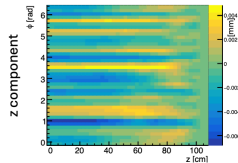
z component of int. distortion in pz plane at r=50.115
