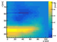
p component of int. distortion in zr plane at p=3.063
