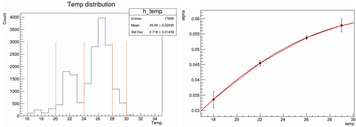
Figure 10: The temperature distribution and temperature range we use to get \alpha(T) (left), and the \alpha distribution (right).
